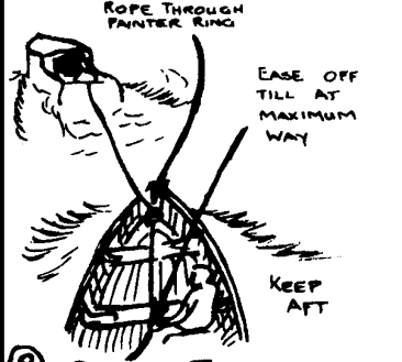
⑧ BEING TOWED
