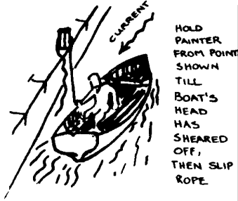
① GETTING AWAY
