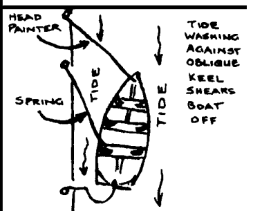
⑭ TO KEEP BOAT OFF
