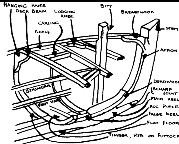
PART FRAME OF MOULDED DECKED BOAT
