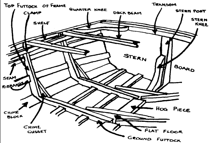
PART FRAME OF CHIME-BUILT BOAT.
